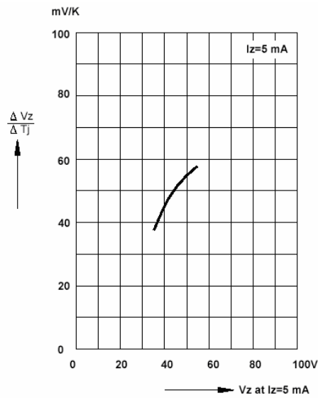
Temperature dependence of Zener voltage
