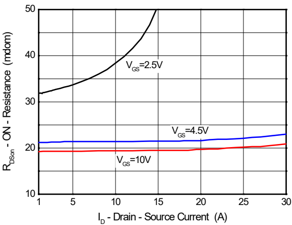
Figure 6. Rdson-Drain Current
