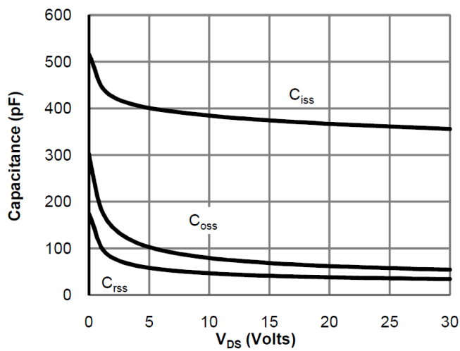
Figure 7. Capacitance Characteristics
