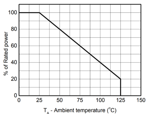
Figure5: Power derating vs Ambient temperature
