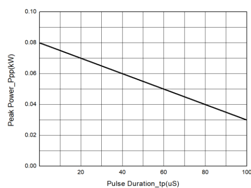
Figure6: Peak Pulse Power vs Pulse Time
