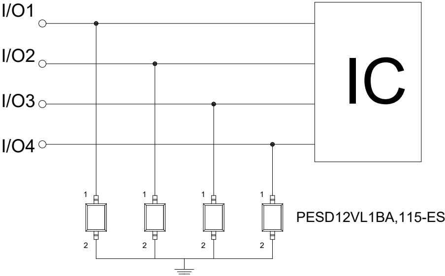
Typical Interface Application
