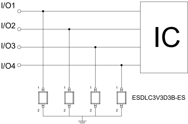
Typical Interface Application
