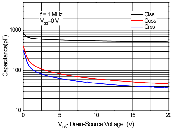
Figure 3. Capacitance Characteristics
