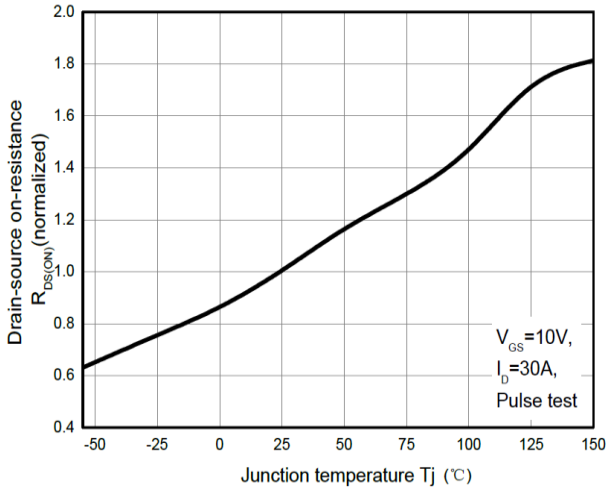
Figure 6.On-Resistance vs.Temperature
