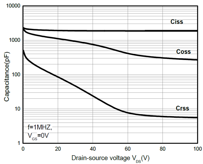
Figure 7. Capacitance Characteristics
