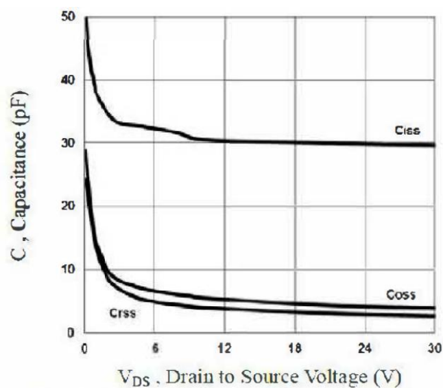
Fig.3 Capacitance Characteristics
