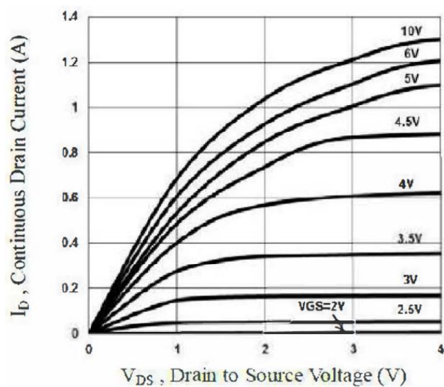
Fig.1 Output Characteristics
