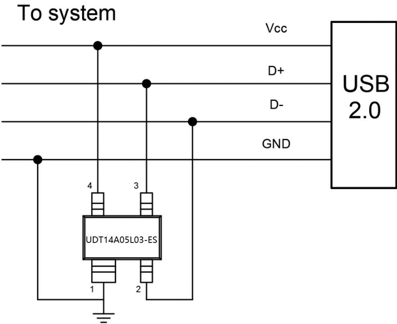
Typical Interface Application
