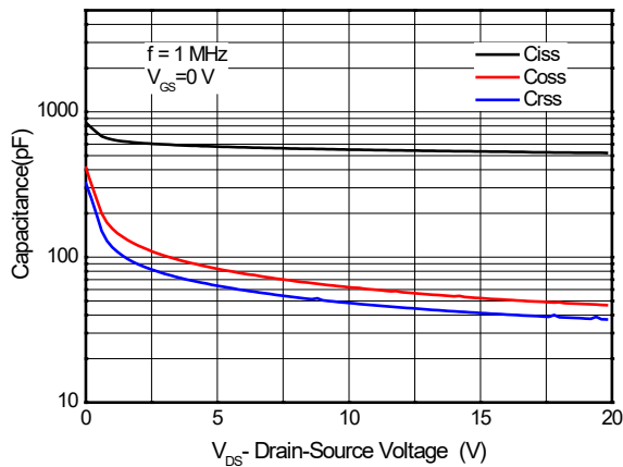
Figure 3. Capacitance Characteristics
