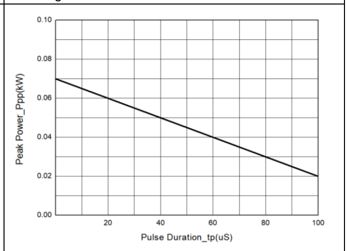
Figure6: Peak Pulse Power vs Pulse Time
