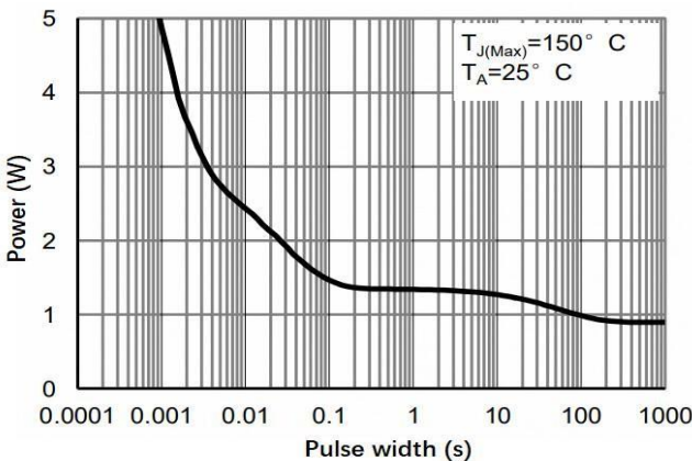
Figure8. Pulse Power Rating Junction-to Ambient
