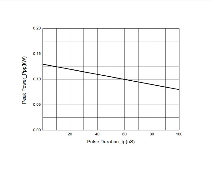
Figure5: Peak Pulse Power vs. Pulse Time
