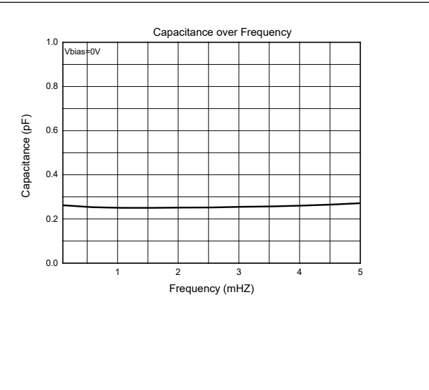
Figure6: Capacitance over Frequency
