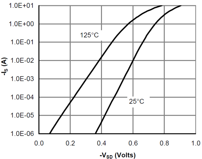
Figure 6: Body-Diode Characteristics
