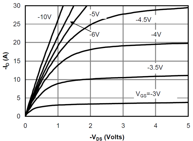
Fig 1: On-Region Characteristics
