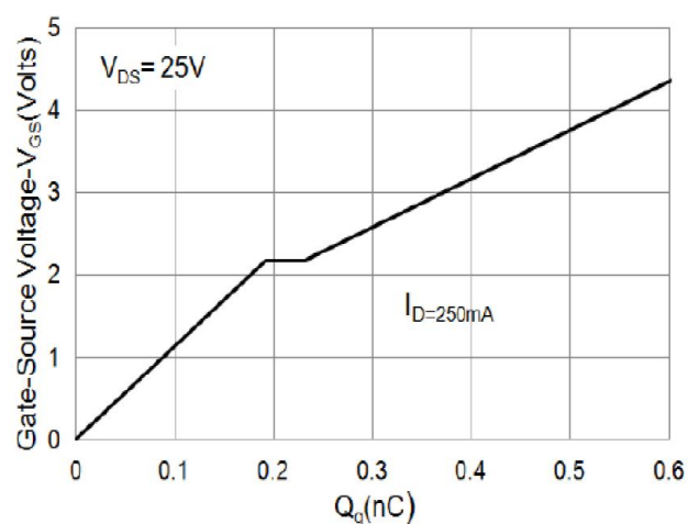
Fig.7 Gate-Charge Characteristics
