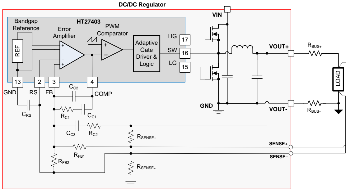
图 37. HT27403 Output Remote Sense and Voltage Control Loop
