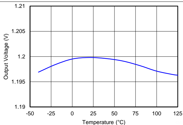
图 5. Temperature Regulation
