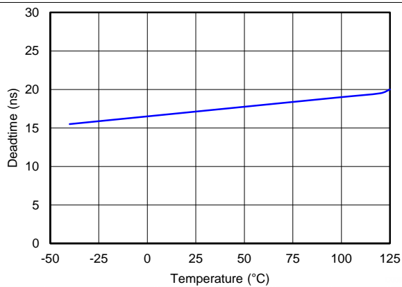
图 9. Deadtime vs. Temperature
