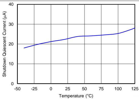
图 7. Shutdown Quiescent Current vs. Temperature
