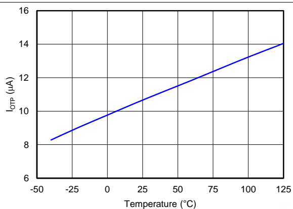
图 11. OTP Current vs. Temperature
