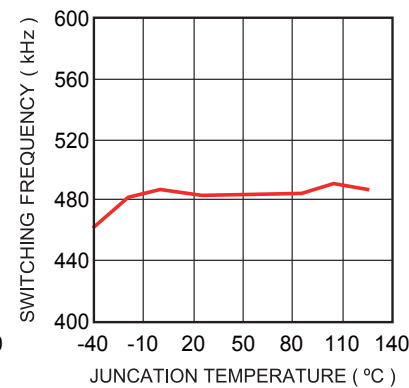
Frequency vs. T_J
