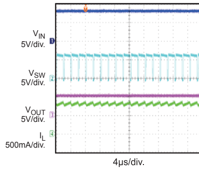
Steady State
