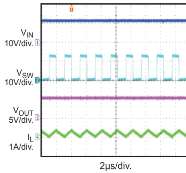
Steady State
