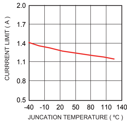
Current Limit vs. T_J
