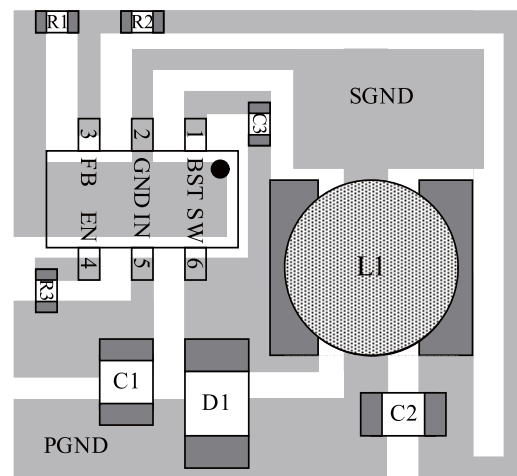
Figure 2: PCB Layout
