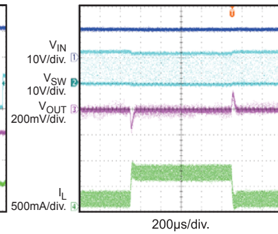
Load Transient
