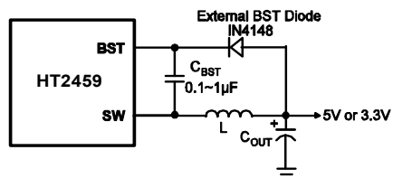
Figure 3: Optional Bootstrap Diode for Enhanced Efficiency
