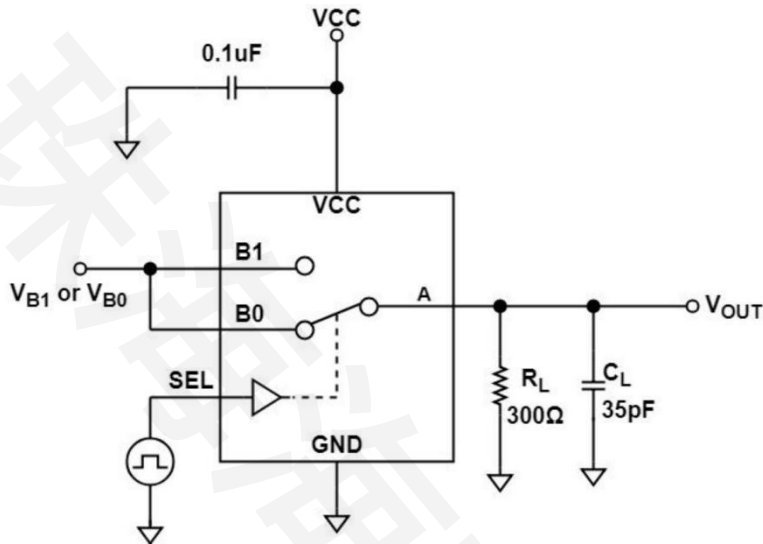
Test Circuit 3. Break-Before-Make Time Delay, t_b
