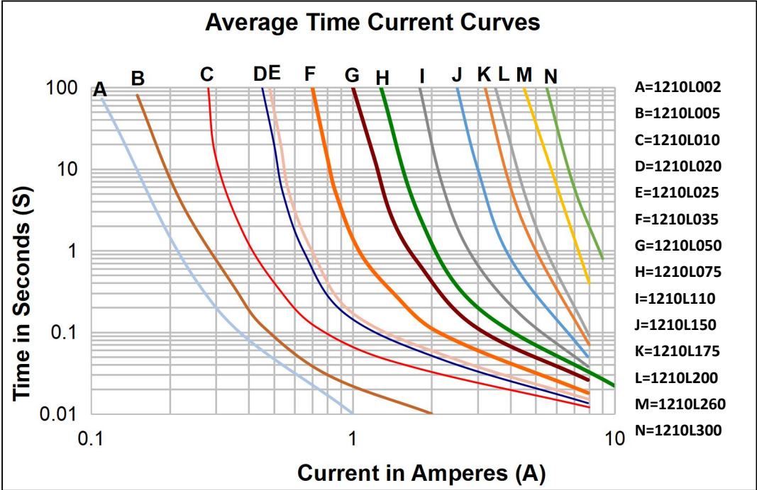
Typical Time-to-Trip at 25°C/25°C跳闸保护时间曲线表
