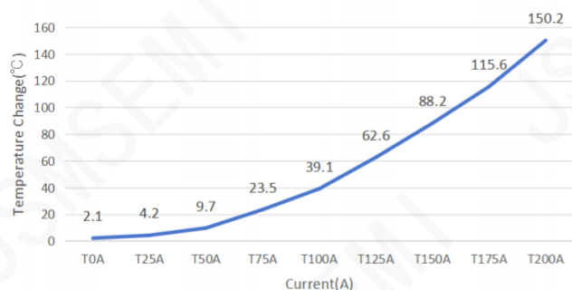
Thermal curve
