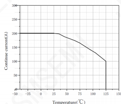
Derating curve
