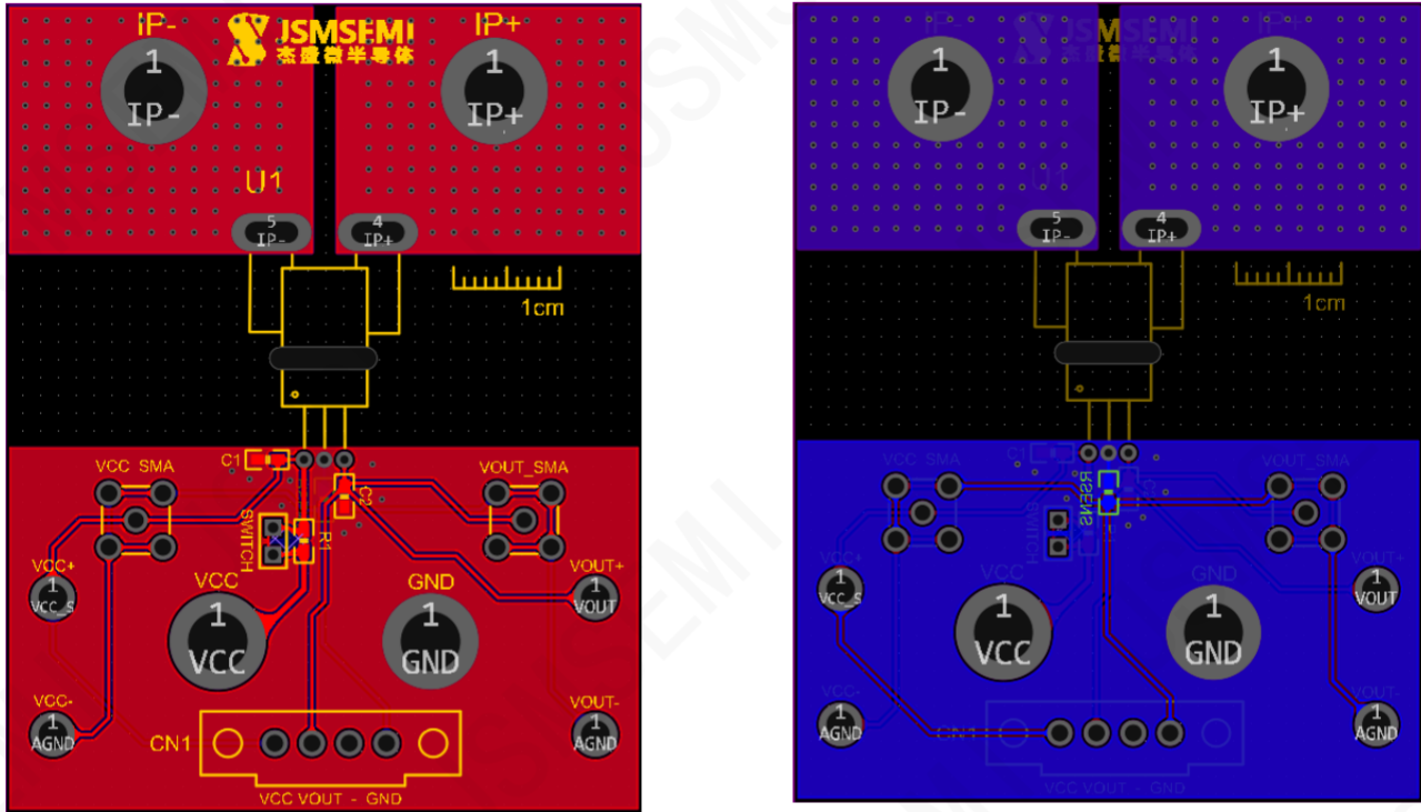
FigDemo board
