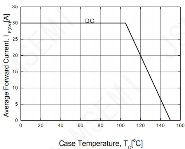
Figure 4. Power Derating
