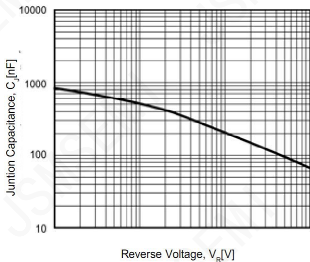
Figure 3. Junction Capacitance
