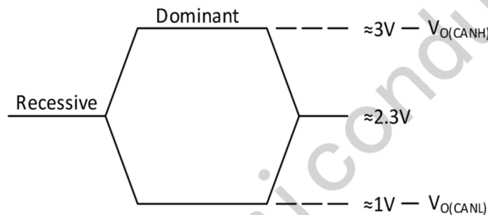
Figure 2. Bus Logic State Voltage Definitions
