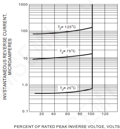
Fig.3-TYPICAL REVERSE CHARACTERISTIC
