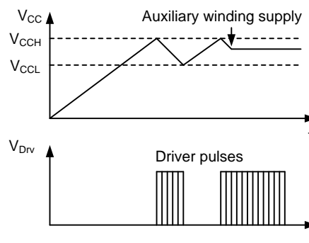
Figure 2: V_{CC} UVLO
