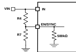
Figure 12: Adjustable UVLO using EN/SYNC Divider
