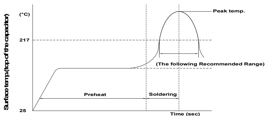
TEMPERATURE PROFILE
