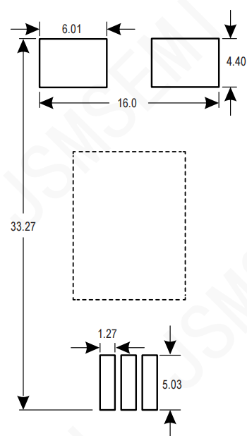
PCB Layout Reference View
