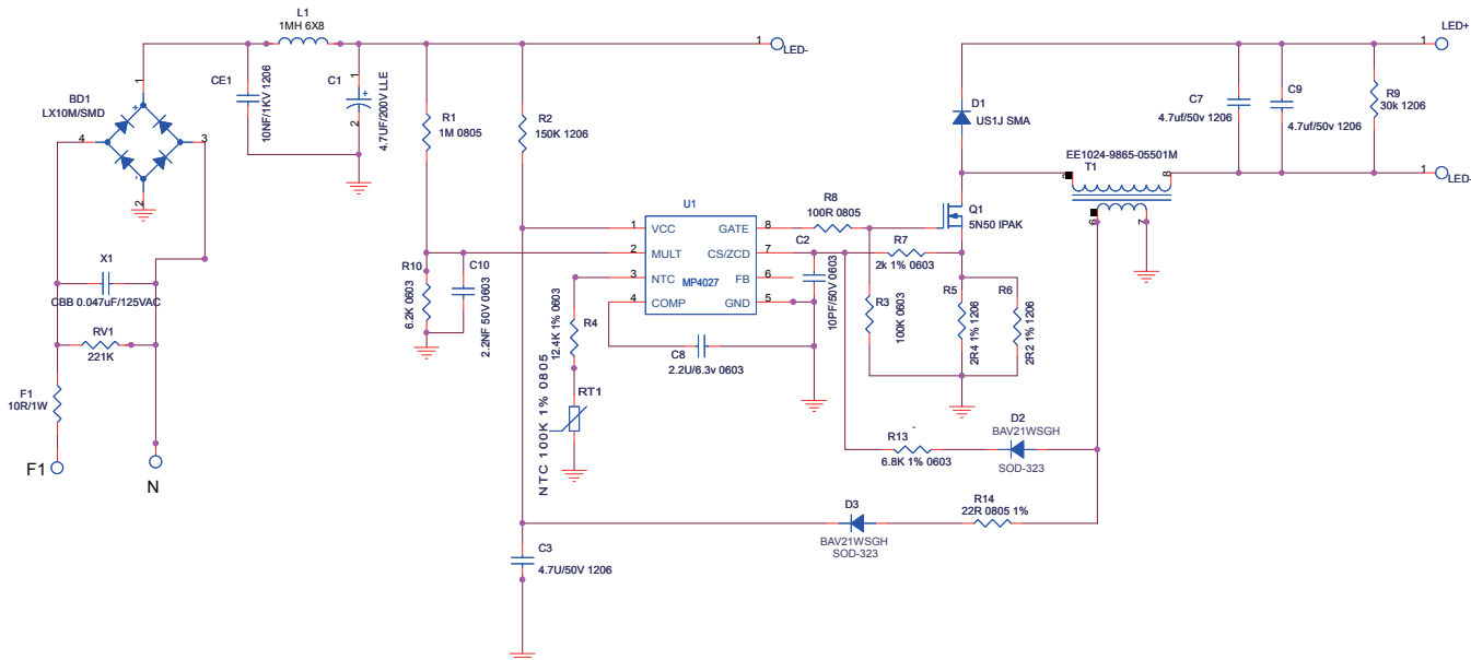
Figure 21: 4W Candle Bulb Driver, 90-132VAC Input, Low-Side Buck-Boost Converter, V_o=23V , I_{LED}=180mA . No PFC requirement, so the input cap is larger than PFC solution, and small output cap can meet the output current ripple requirement
