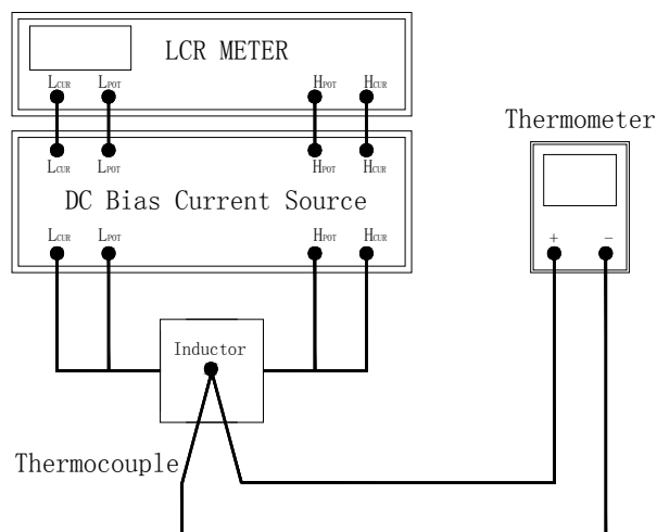
Isat & Irms test schematic diagram
