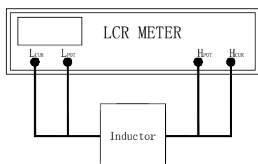
Ls & RDC test schematic diagram
