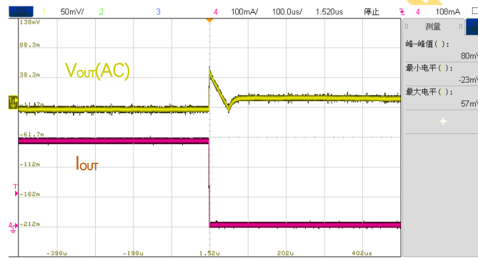
Figure 10. Load Transient 300mA->1mA, V_{IN}=3.3V , V_{OUT}=1.2V
