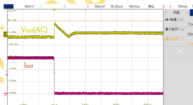
Figure 12. Load Transient 300mA->1mA, V_{IN}=3.3V , V_{OUT}=1.8V
