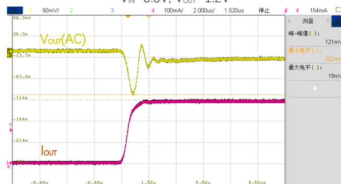
Figure 11. Load Transient 1mA->300mA, V_{IN}=3.3V , V_{OUT}=1.8V
