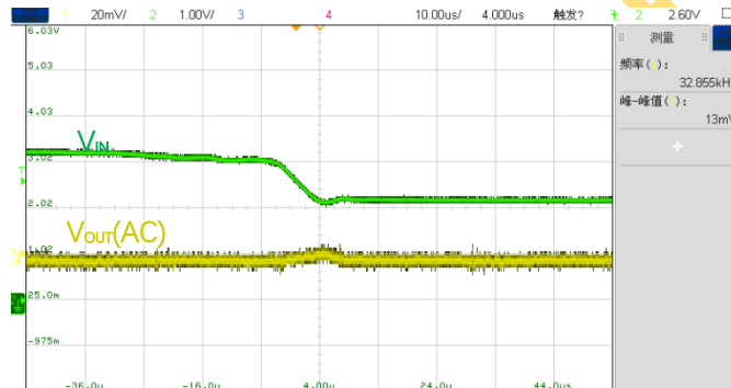
Figure 18. Line Transient V_{IN}=3.2V \rightarrow 2.2V , V_{OUT}=1.2V , I_{OUT}=100mA
