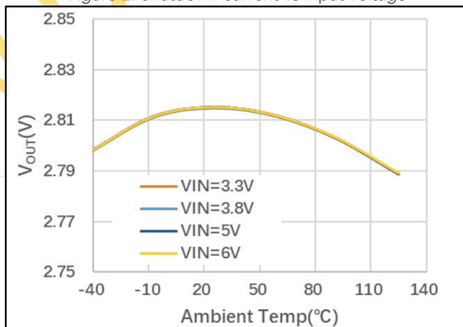
Figure 4. V_{OUT} vs Ambient Temperature, LP3982H-28B5F, I_{OUT}=1\text{mA}
