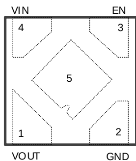
DFN-4 (top view)
