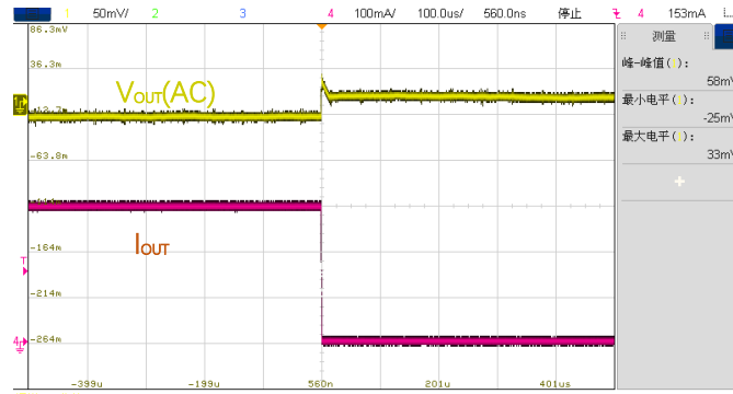
Figure 16. Load Transient 300mA->1mA, V_{IN}=4.3V , V_{OUT}=3.3V
