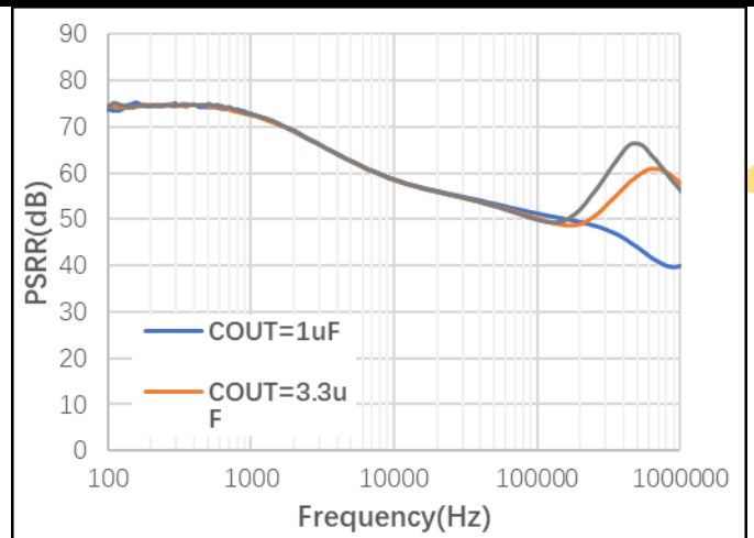
Figure 8. PSRR vs Frequency when V_{OUT}=3.3V I_{OUT}=20mA , V_{IN}=V_{OUT}+1V ,
