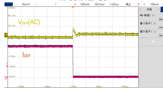
Figure 14. Load Transient 300mA->1mA, V_{IN}=3.8V , V_{OUT}=2.8V
