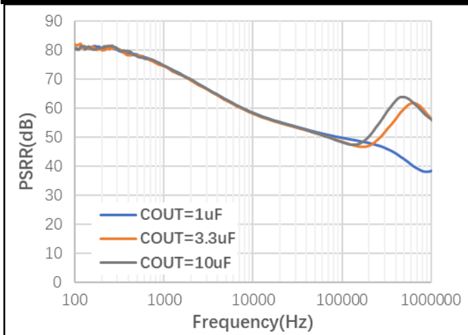
Figure 7. PSRR vs Frequency when V_{OUT}=2.8V I_{OUT}=20mA , V_{IN}=V_{OUT}+1V ,
