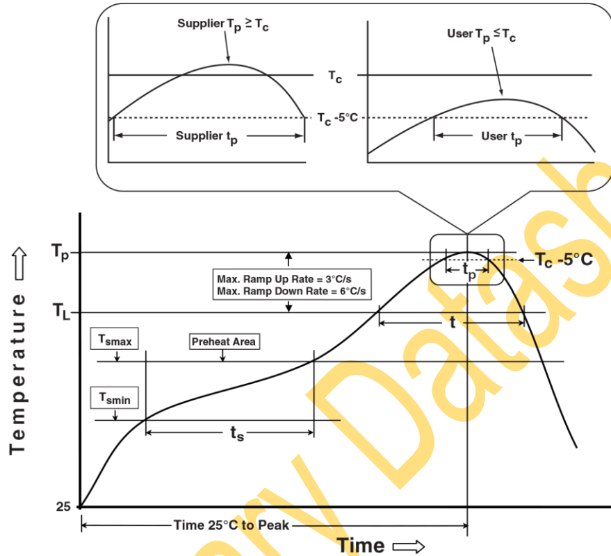
Figure1 Classification Profile (Not to scale)
