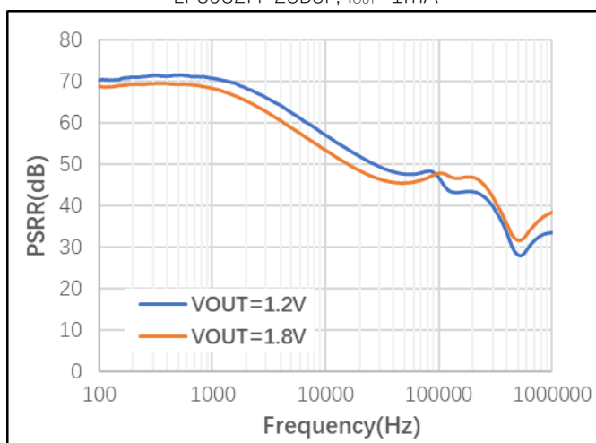
Figure 6. PSRR vs Frequency with V_{OUT}=1.2\text{V}/1.8\text{V} I_{OUT}=20\text{mA} , V_{IN}=V_{OUT}+1\text{V} , C_{OUT}=1\mu\text{F} ,
