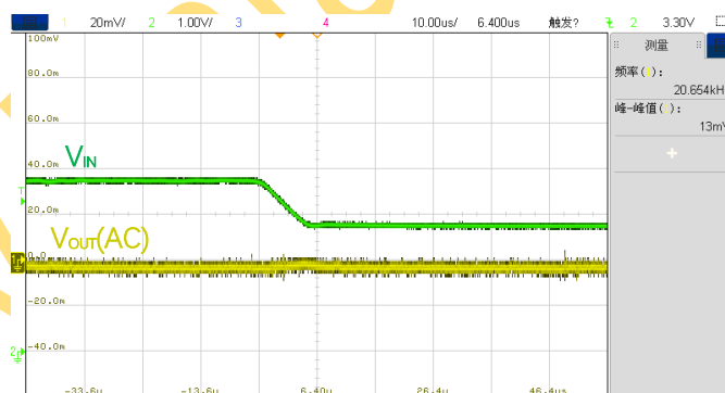
Figure 20. Line Transient V_{IN}=3.8V \rightarrow 2.8V , V_{OUT}=1.8V , I_{OUT}=100mA
