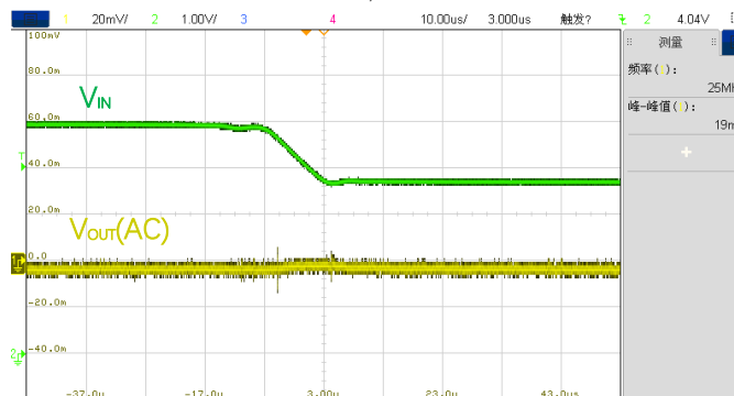
Figure 22. Line Transient V_{IN}=4.8V \rightarrow 3.8V , V_{OUT}=2.8V , I_{OUT}=100mA
