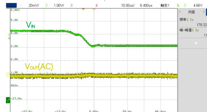
Figure 24. Line Transient V_{IN}=5.3V \rightarrow 4.3V , V_{OUT}=3.3V , I_{OUT}=100mA
