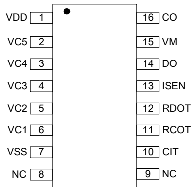
SOP16, SSOP16 (top view)
