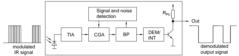
Fig.1 Block Diagram
