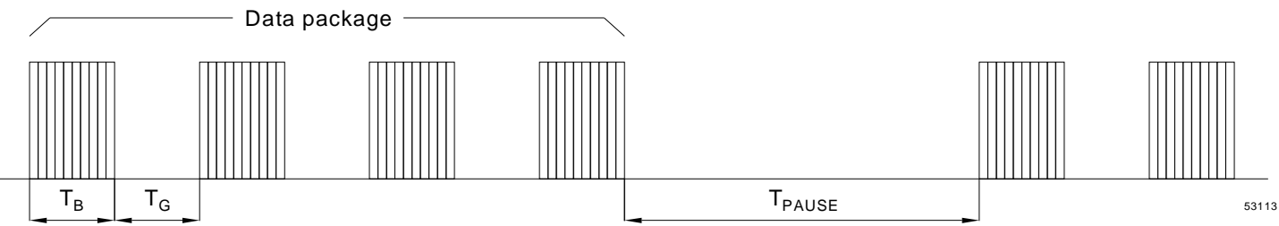
Fig.7: general IR data structure
