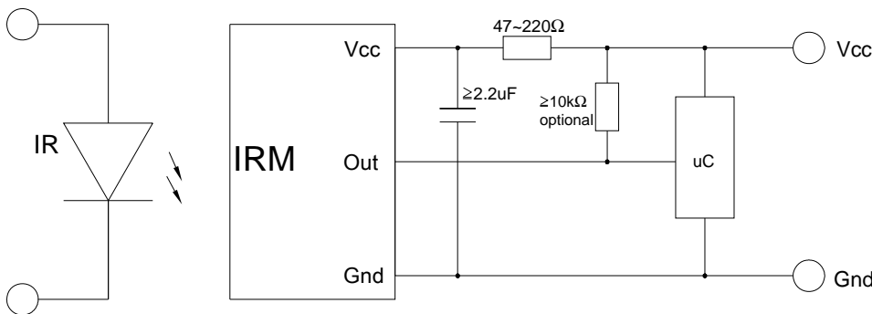
Fig.6: application circuit
