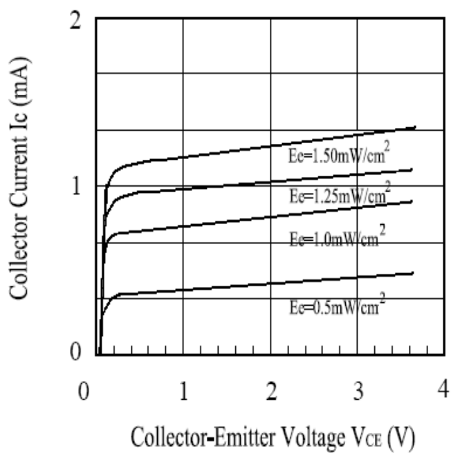
Fig.4 Collector Current vs. Collector-Emitter Voltage
