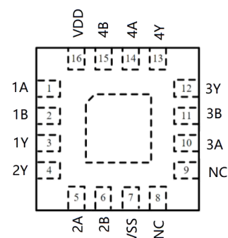
QFN-16 3*3
