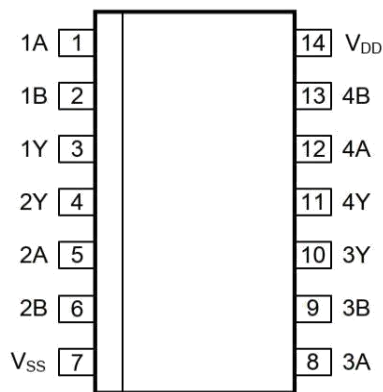
DIP-14/SOP-14/TSSOP-14
