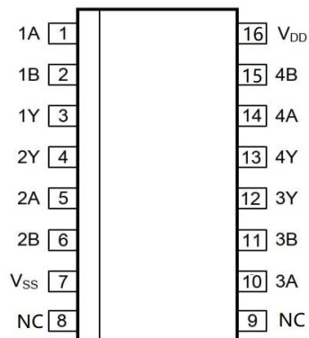
QSOP-16
