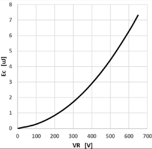
Figure 7. Capacitance Stored Energy
