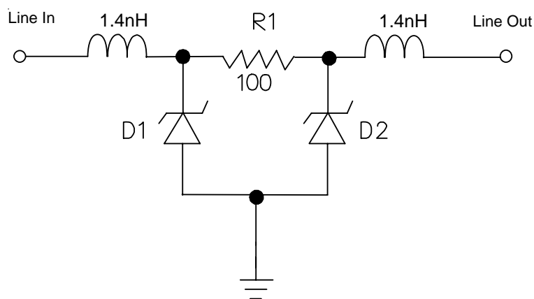
EClamp2378K Spice Model
