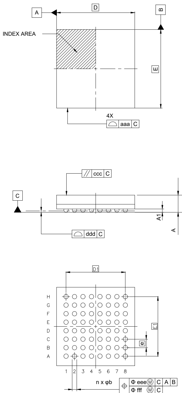
Figure 2.4 BGA 64-pin
