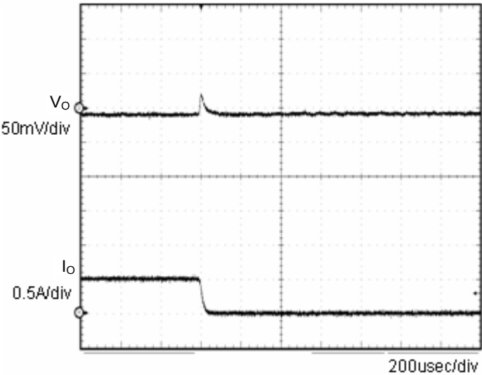
Fig.4 Transient Response (0.5→0A) Co=1μF
