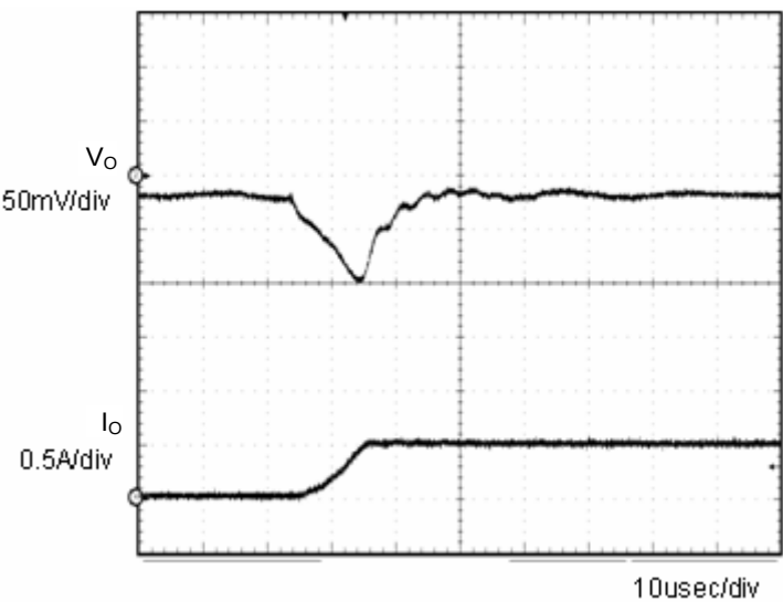
Fig.3 Transient Response (0→0.5A) Co=1μF
