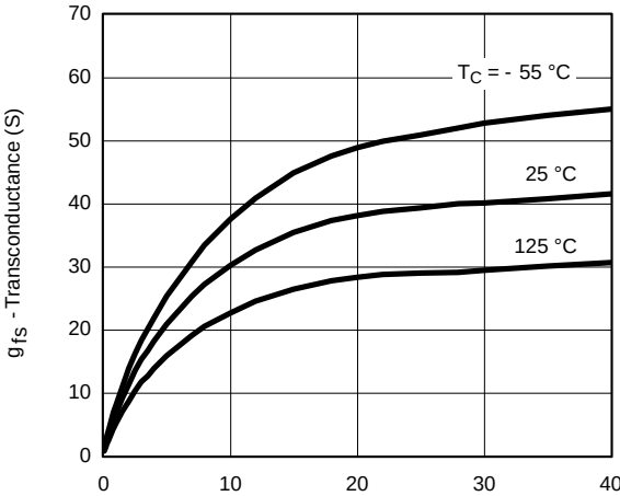
Transconductance
