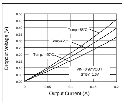
Fig. 66 Dropout Voltage
