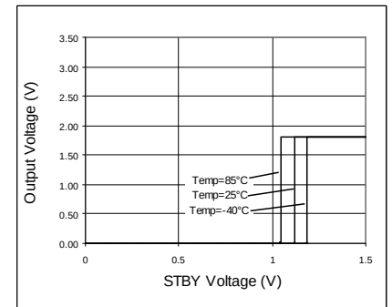
Fig. 42 STBY Threshold
