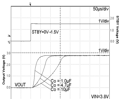
Fig. 115 Start Up Time I_{out} = 0\text{mA}
