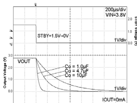
Fig. 119 Discharge Time I_{out} = 0\text{mA}
