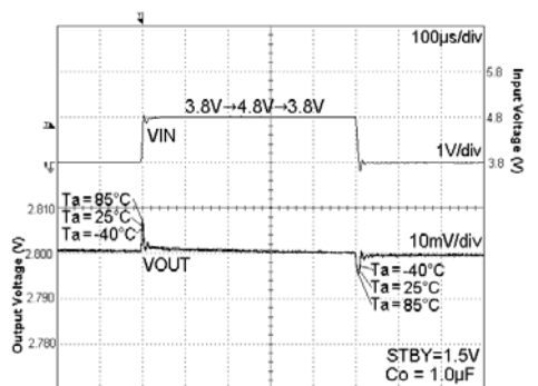
Fig. 120 VIN Response I_{out} = 10\text{mA}
