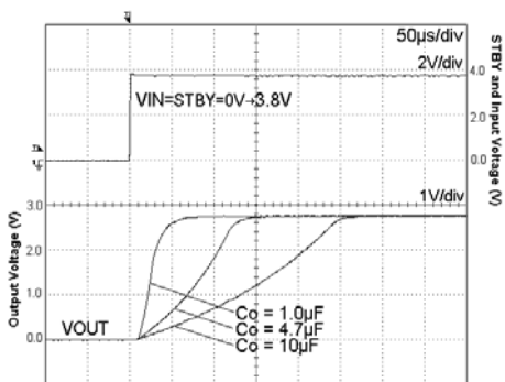
Fig. 118 Start Up Time (STBY=VIN) I_{out} = 200\text{mA}
