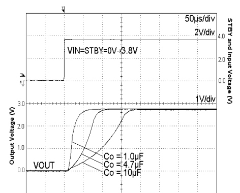
Fig. 117 Start Up Time (STBY=VIN) I_{out} = 0\text{mA}
