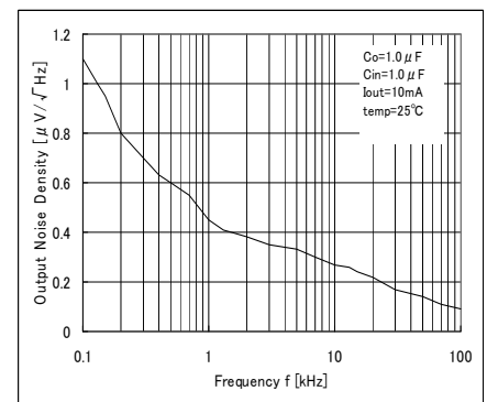
Fig. 77 Output Noise Spectrl Density VS Freq.
