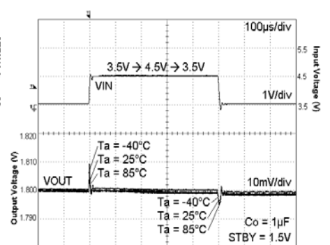
Fig. 62 VIN Response I_{out} = 10\text{mA}
