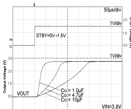
Fig. 116 Start Up Time I_{out} = 200\text{mA}
