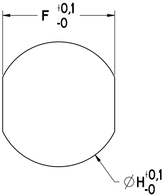
PANEL CUTOUT
