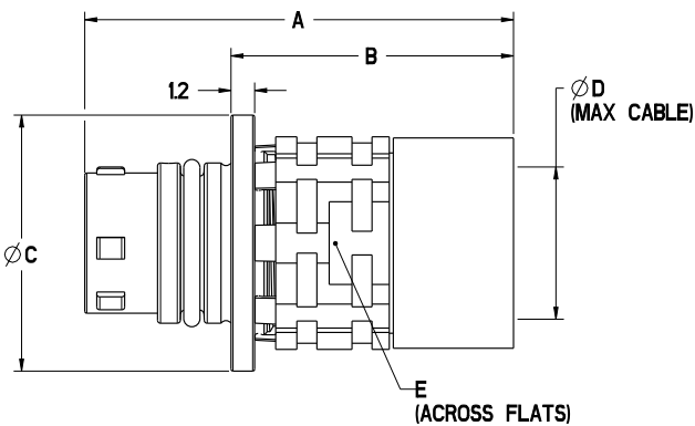
Breakaway Plug
