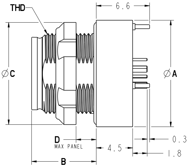
PCB
