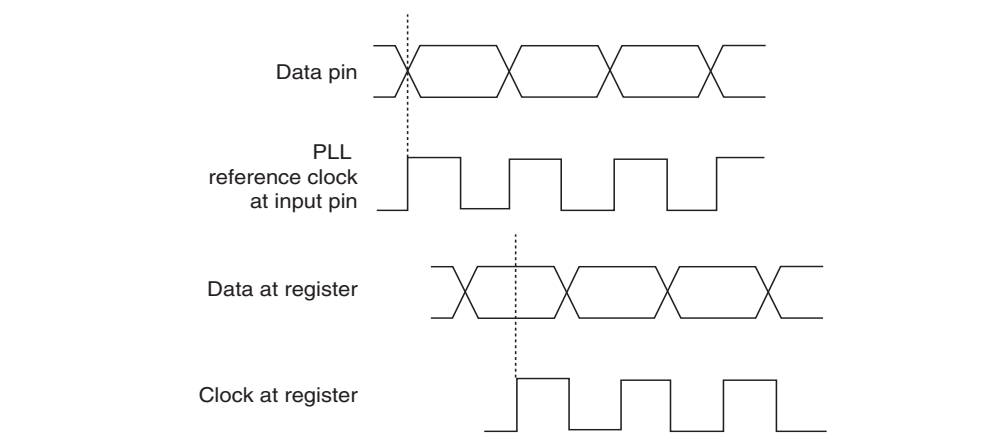
Figure 5-25. Source-Synchronous Mode for LVDS Compensation for Arria II Devices
