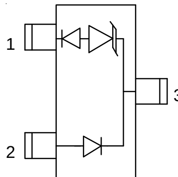
SOT-23 3L (Top View)
