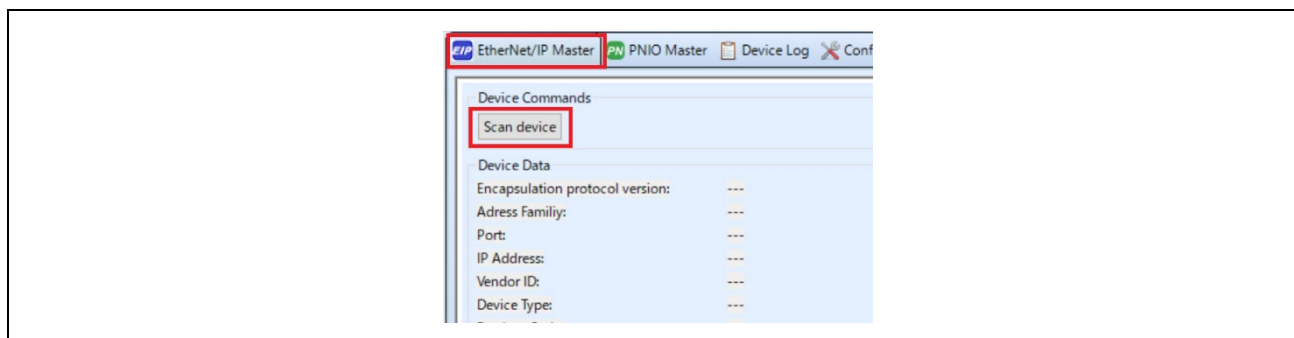
Figure 3-36 Scan device
