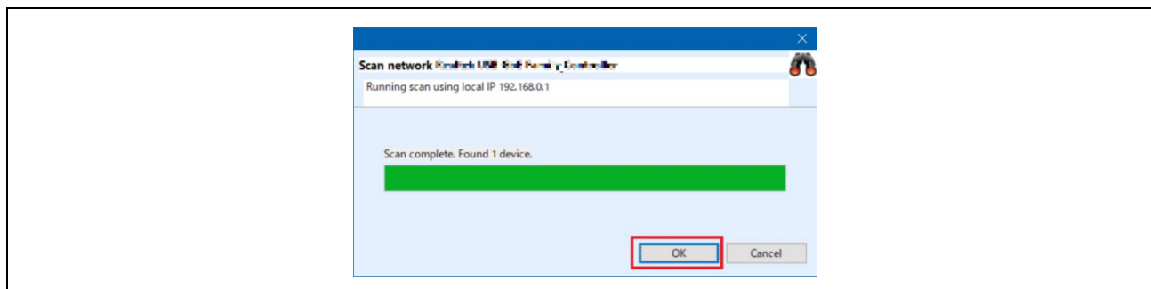
Figure 3-17 Scan completed
