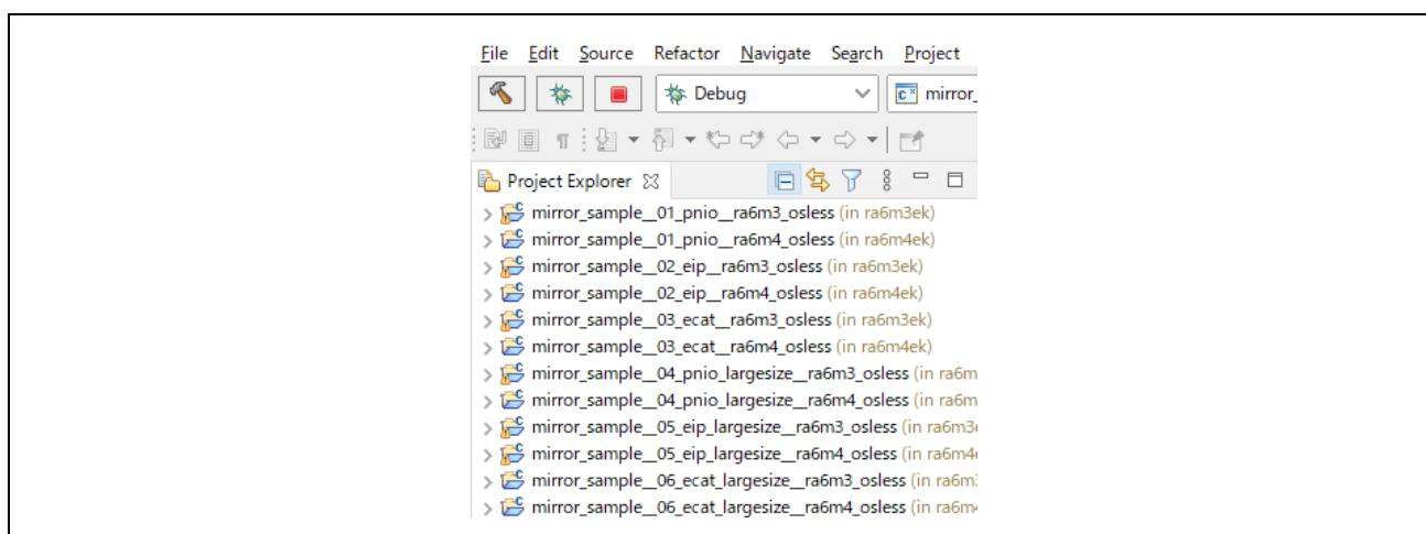
Figure 3.7 Imported projects
