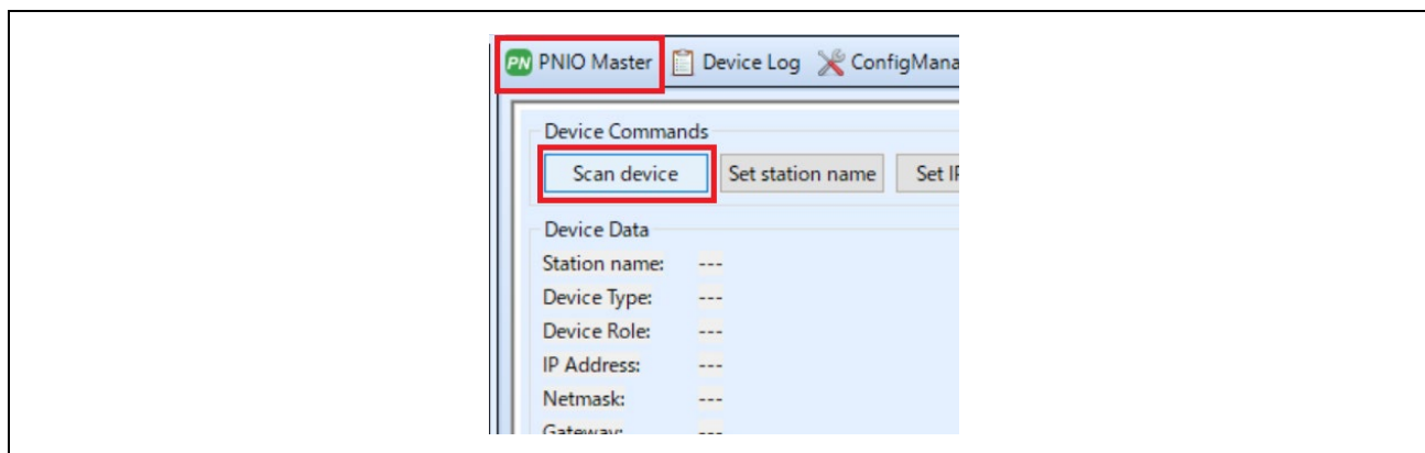
Figure 3-22 PNIO Master
