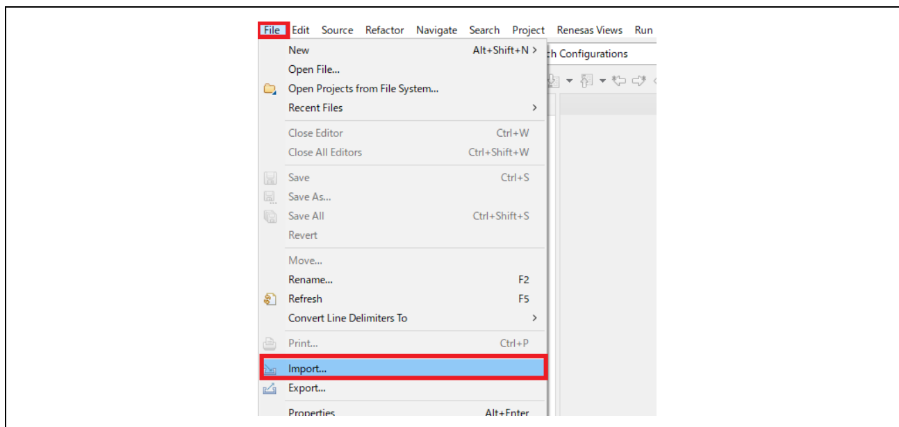
Figure 3.4 Import
