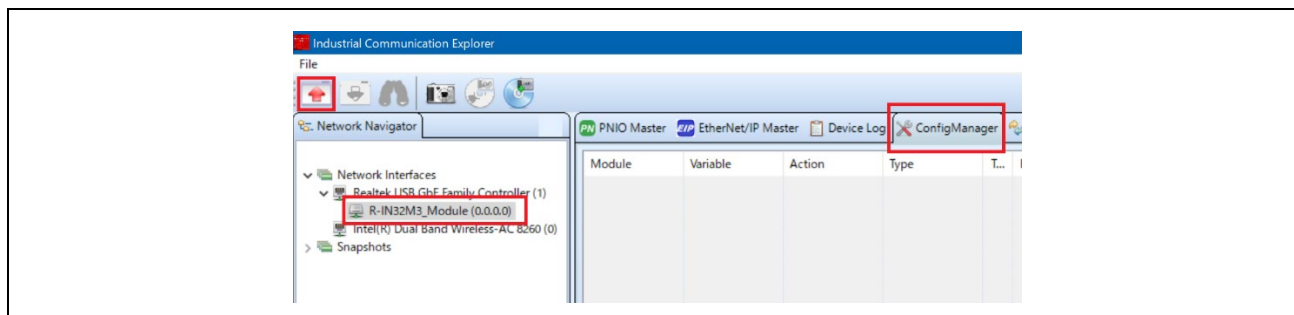
Figure 3-33 ConfigManager
