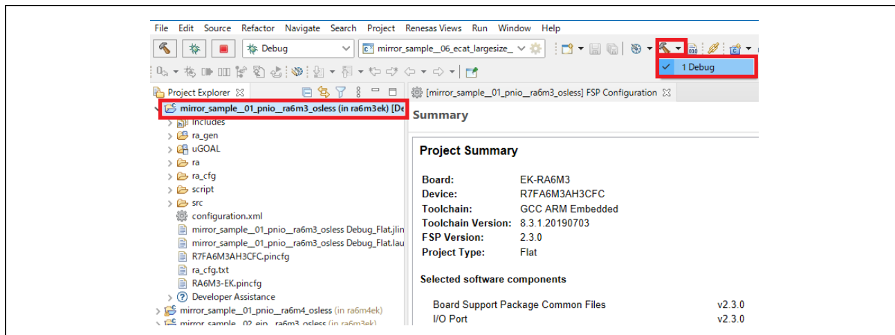
Figure 3.10 Build project
