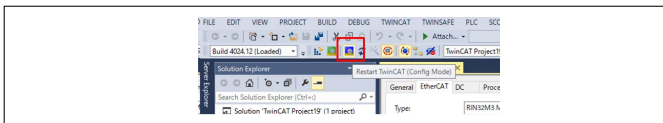
Figure 3.59 re-connect TwinCAT
