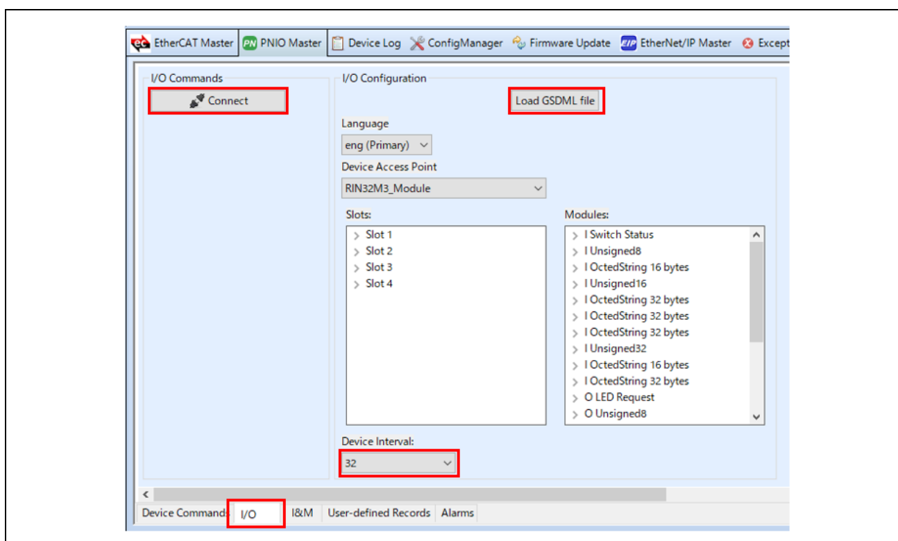
Figure 3-24 GSDML
