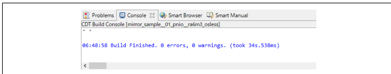
Figure 3.11 Build finished
