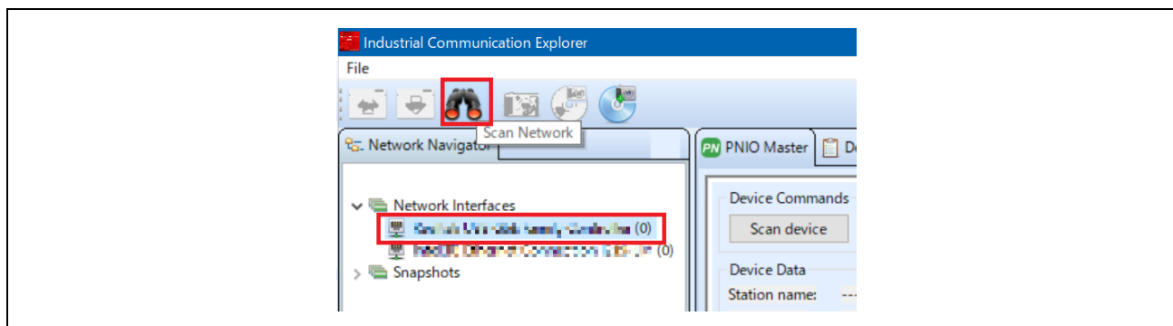
Figure 3-16 Scan network
