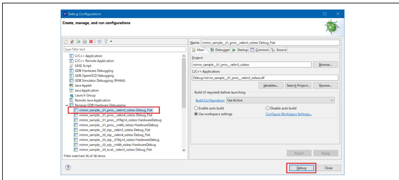
Figure 3.13 Debug start
