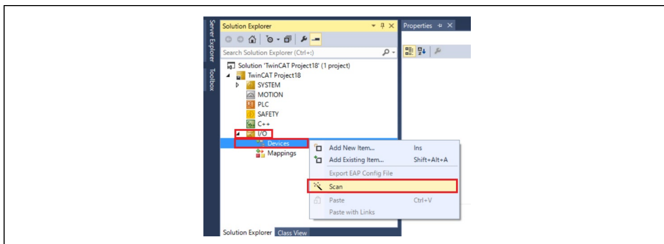
Figure 3-45 Scan network
