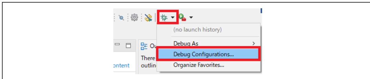
Figure 3.12 Debug Configurations
