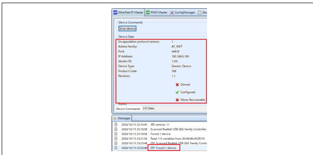
Figure 3-37 Device Data
