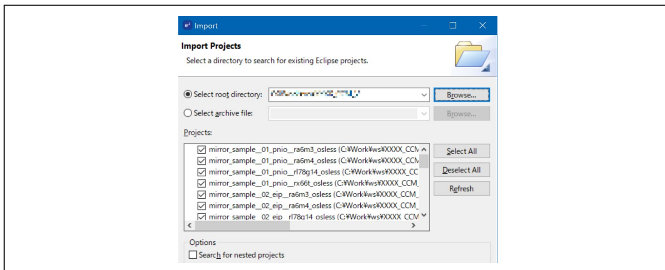
Figure 3.6 Import Projects
