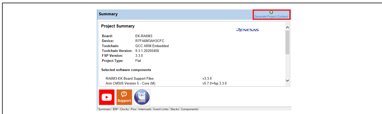
Figure 3.9 Generate code
