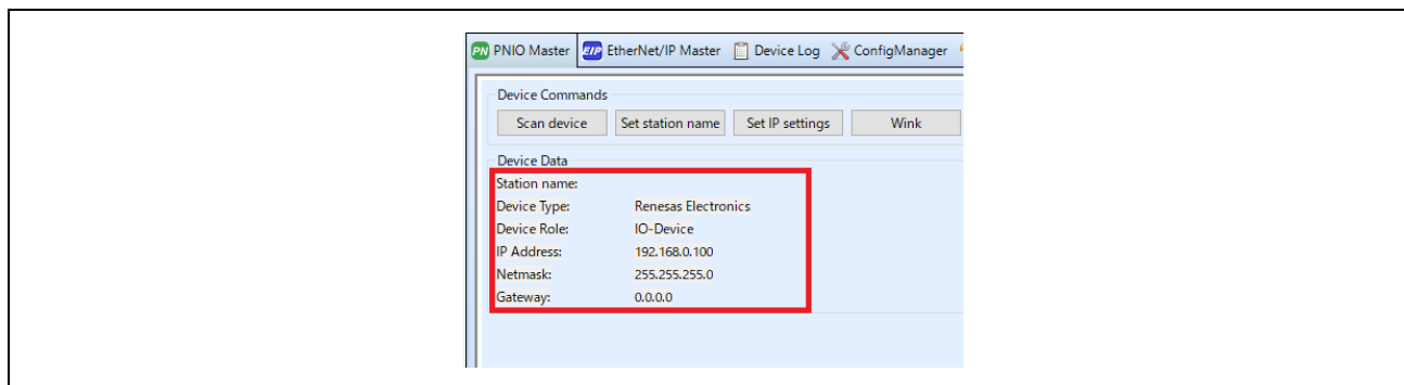
Figure 3-23 Device Data
