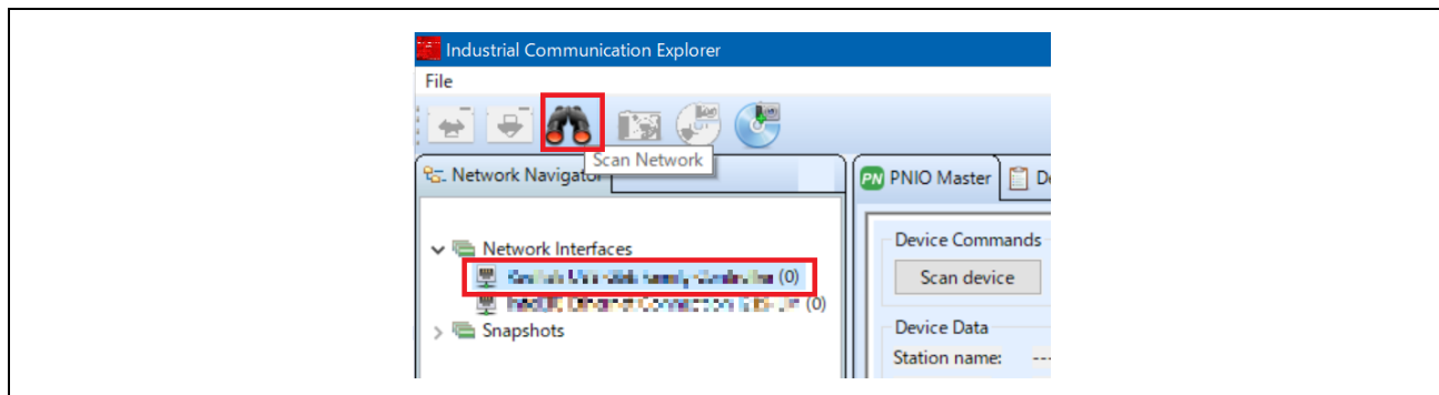
Figure 3-30 Scan network
