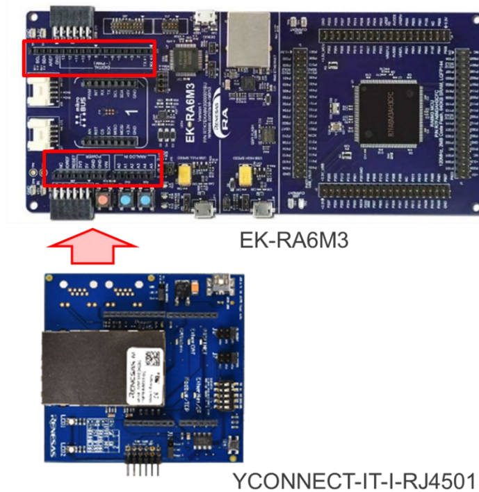
Figure 2-2 Arduino™ Connection
