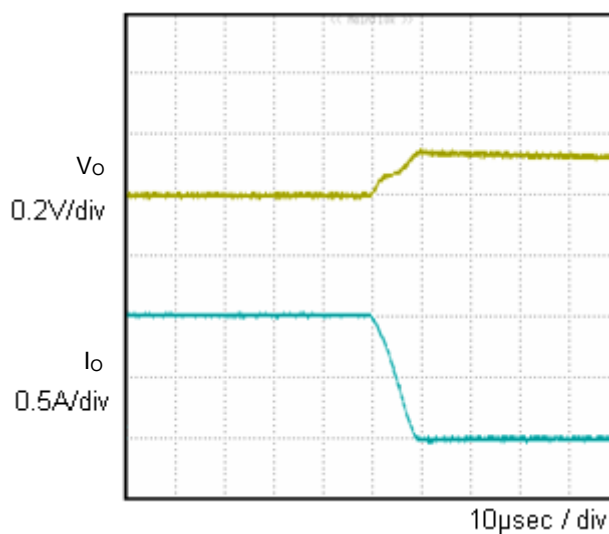
Fig.4 Transient Response(1.0→0A) \text{Co}=1.0\mu\text{F}
