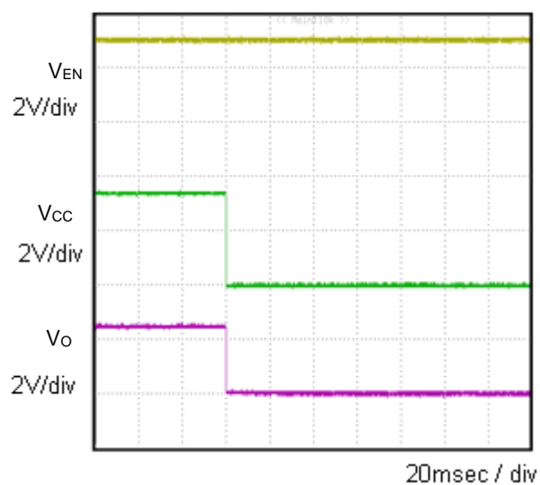
Fig.6 OFF sequence 1 \text{Co}=1.0\mu\text{F}
