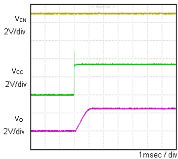
Fig.5 Input sequence1 \text{Co}=1.0\mu\text{F}
