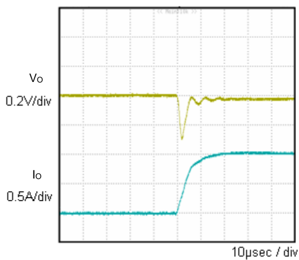
Fig.3 Transient Response(0→1.0A) \text{Co}=1.0\mu\text{F}
