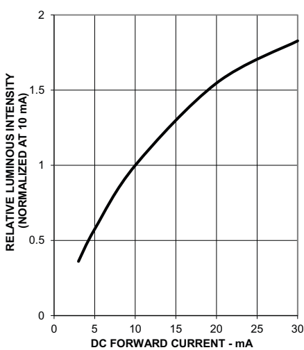
Figure 3: Relative Luminous Intensity vs. DC Forward Current
