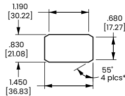
MOUNTING HOLE (Nylon Snap-in Brackets) Panel Thickness: .030 min. - .250 max. * Angled corners are suggested for optimum fit. Standard rectangular cutout is acceptable.
