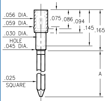
170X-X-17-XX-30-XX-02-0 Press-fit in .057 mounting hole
